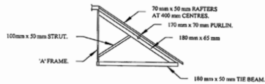
DETAIL OF HIP SUPPORT
