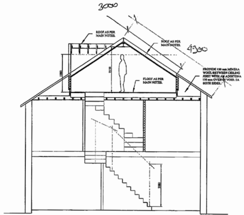
SECTION THROUGH STAIRS SCALE 1:50
