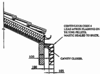
DETAIL OF BOUNDARY GUTTER (SCALE: 1:20)
