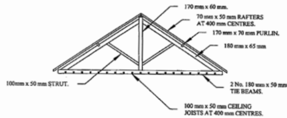
DETAIL OF 'A' FRAME
