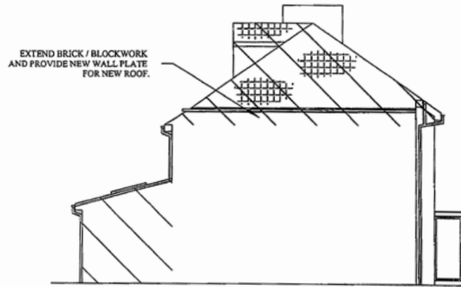
VIEW ON ARROW D
