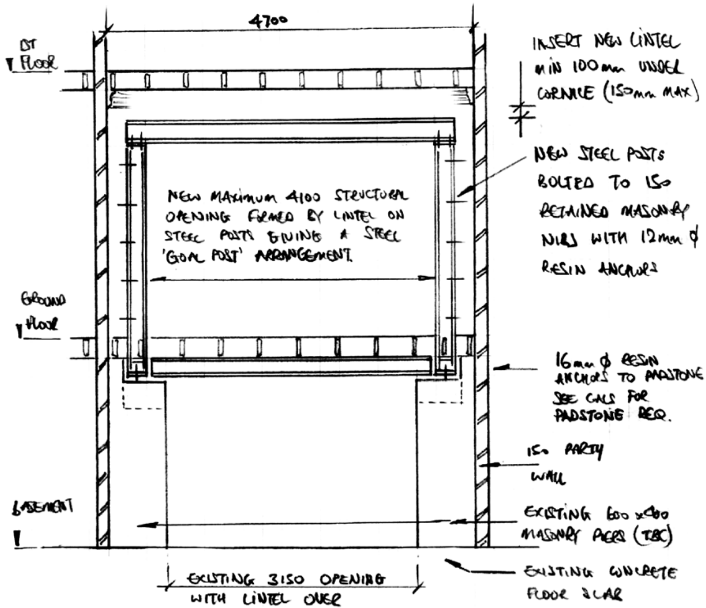
ELEVATION ON PROPOSED NEW OPENING (NTJ)
